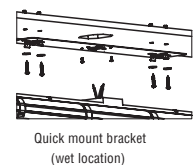
J-Box & Quick Mount Bracket Mount (JM, QMBWBS14)
