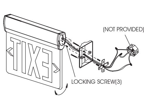
FIG. 3 SURFACE END MOUNTING
