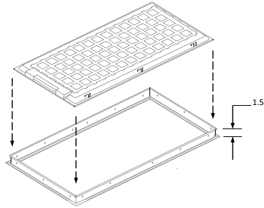
FMK-24 (Flange Mount Kit)
