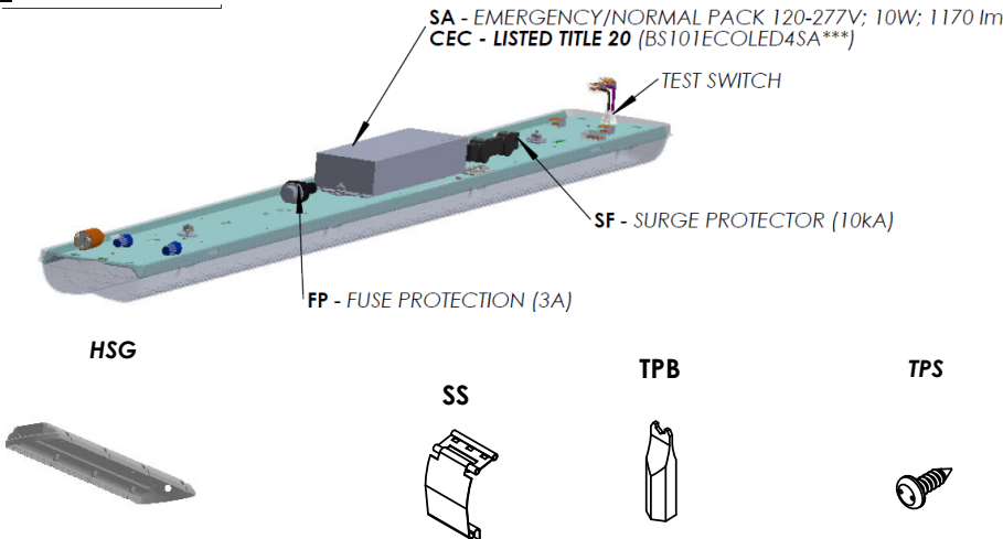
FSP-221B-S FAMILY
