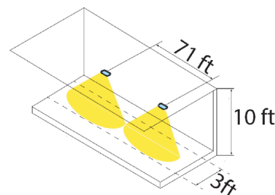
CEILING MOUNT LED ORIENTATION (145° / 145°)
